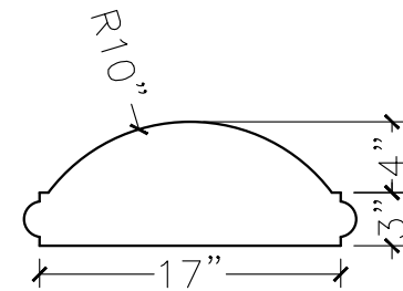
SECTION VIEW
