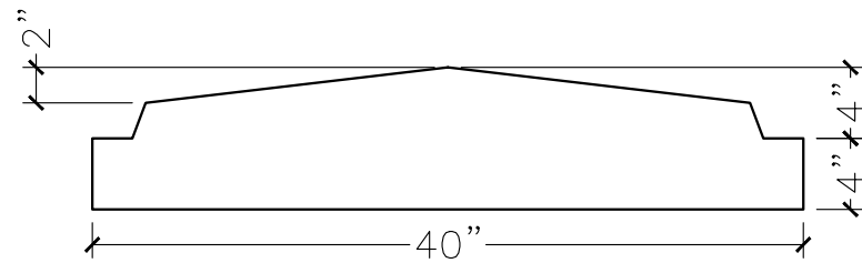
SECTION VIEW
