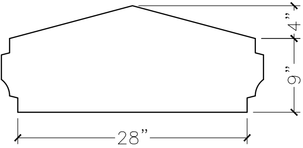
SECTION VIEW
