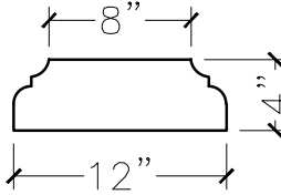
SECTION VIEW
