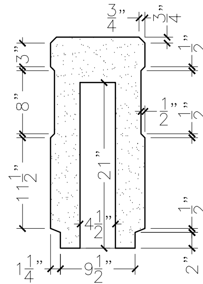
SECTION VIEW
