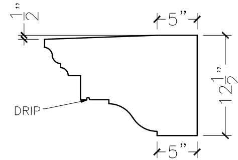
SECTION VIEW
