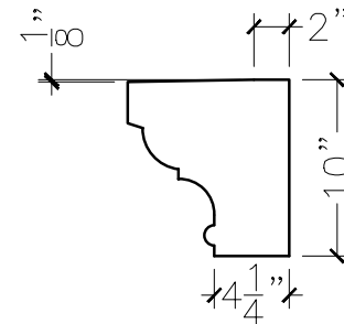
SECTION VIEW
