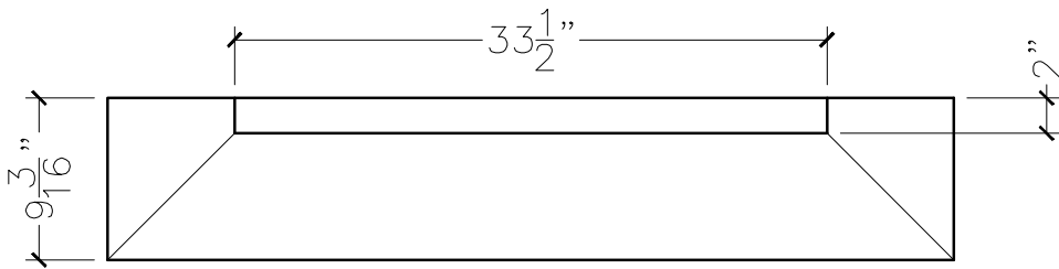
TOP VIEW
