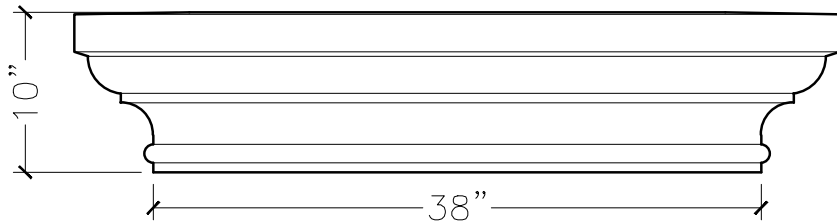
FRONT VIEW
