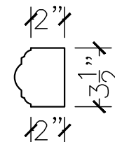
SECTION VIEW
