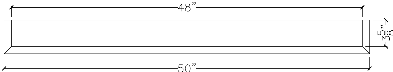
TOP VIEW
