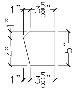
SECTION VIEW
