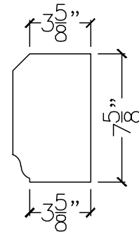
SECTION VIEW
