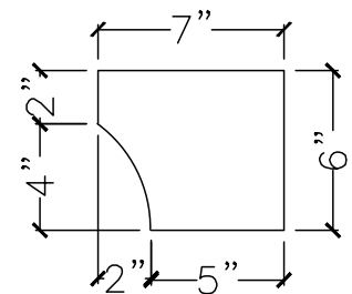
SECTION VIEW
