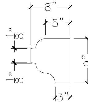
SECTION VIEW
