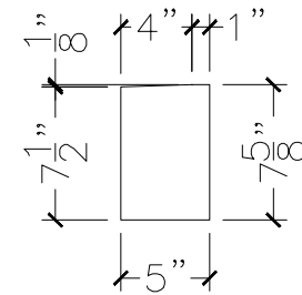
SECTION VIEW
