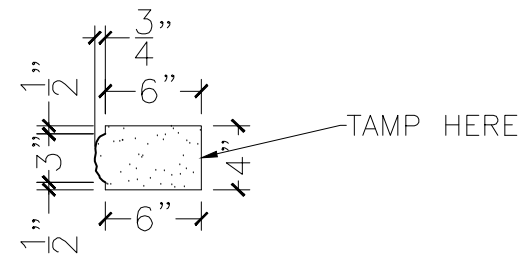
SECTION VIEW
