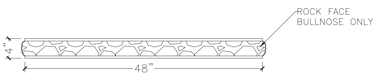
FRONT VIEW
