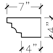
SECTION VIEW
