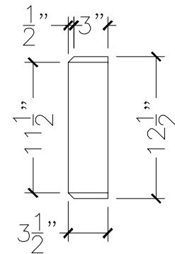
SECTION VIEW
