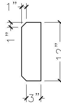
SECTION VIEW
