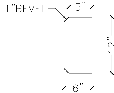
SECTION VIEW
