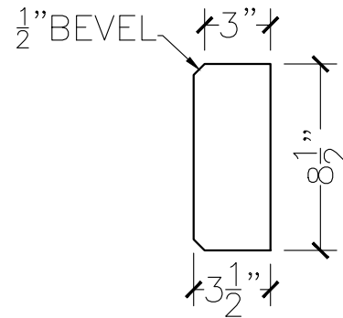
SECTION VIEW
