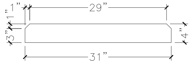
SECTION VIEW
