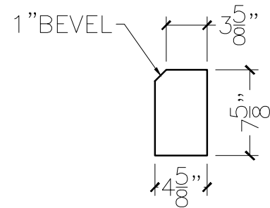
SECTION VIEW
