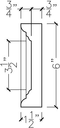
SECTION VIEW
