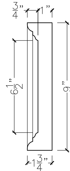
SECTION VIEW
