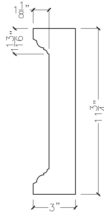
SECTION VIEW
