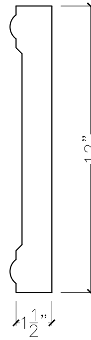
SECTION VIEW
