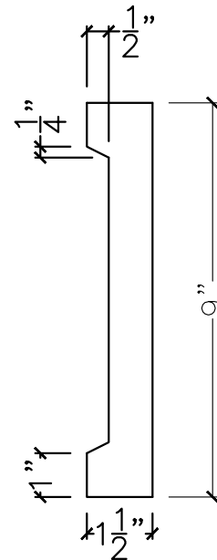
SECTION VIEW
