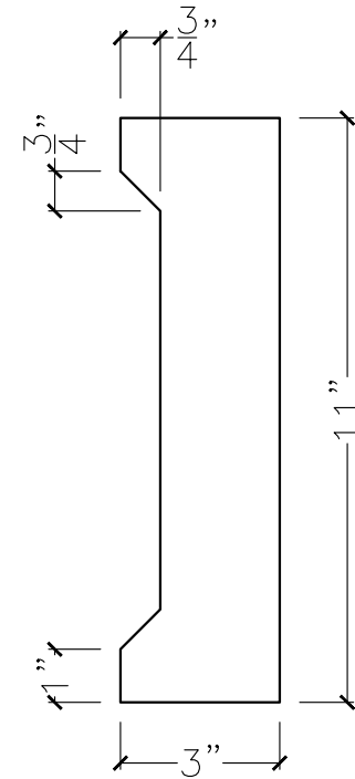
SECTION VIEW
