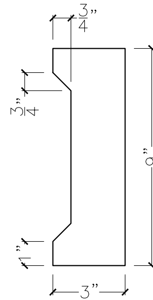
SECTION VIEW
