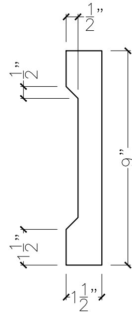
SECTION VIEW
