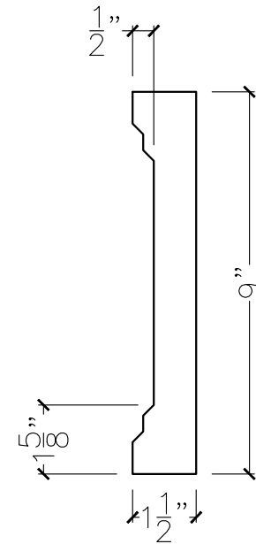
SECTION VIEW
