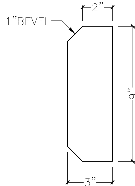
SECTION VIEW
