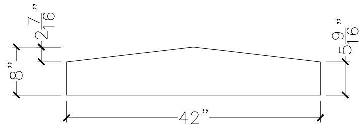
SECTION VIEW
