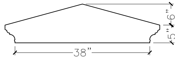
SECTION VIEW
