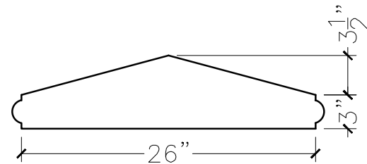
SECTION VIEW
