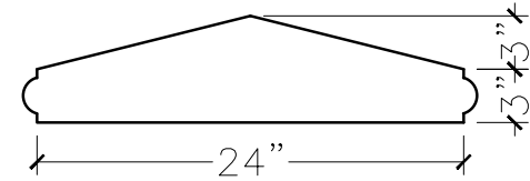
SECTION VIEW
