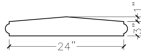
SECTION VIEW
