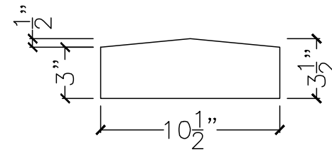
SECTION VIEW
